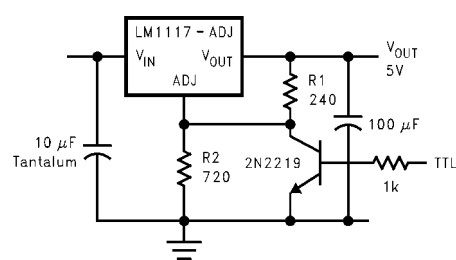
5V Logic Regulator with Electronic Shutdown*
