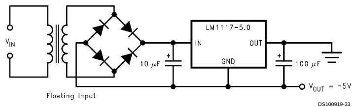
Low Dropout Negative Supply
