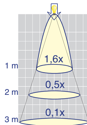
KEPL120908 (70°) 3 METER
